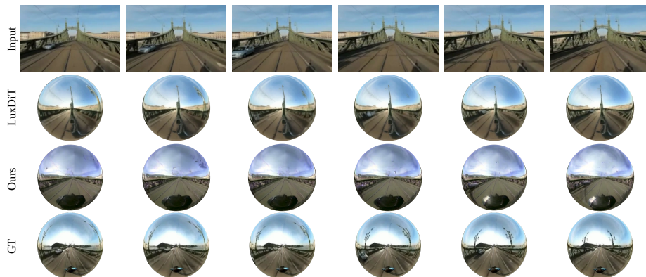
Fig. B: Qualitative comparison with LuxDiT [3]. Using results from their official project page, we demonstrate that V-LITE captures superior lighting details. Notably, V-LITE successfully infers the presence of an out-of-view human in the generated chrome ball by actively reasoning about the cast shadow in the input video.
