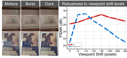
Fig. 9: Left: Comparison with state-of-the-art burst method [7] on their dataset. Our method achieves comparable or better quality while running 60\times faster. Right: Performance across different viewpoint shift levels on DUALREF-R test set, demonstrating our method’s robustness compared to burst approaches.
