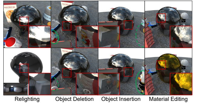
Figure 6. Our explicit representation of geometry, material, and incident lighting in the Gaussian point cloud enables various editing applications. Insets have been brightened for clarity.
