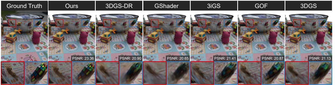
Figure 1. Our SpecTRe-GS effectively captures the appearance of reflectors with highly specular surfaces, even in the presence of nearby objects. In the real-world scene shown above, it performs favorably against previous methods [13, 15, 30, 39, 42], both visually (as the highlighted reflections within the insets) and quantitatively (with PSNR values within the reflective region annotated in the corners).
