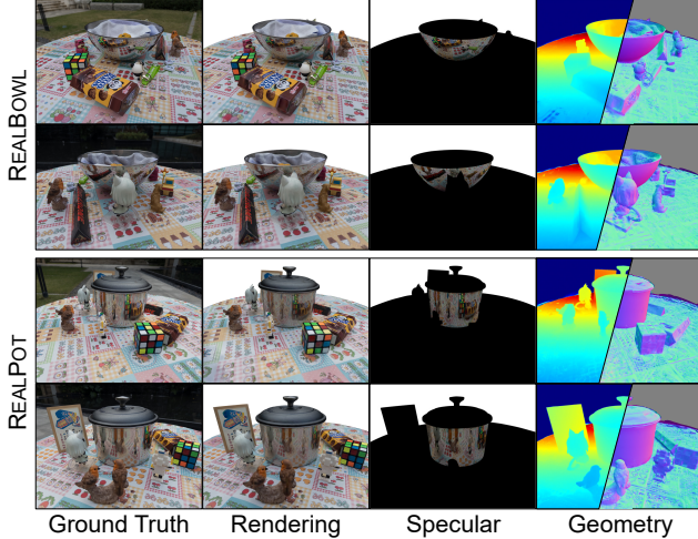
Figure 5. Our reconstruction results on two real-world scenes. SpecTRe-GS accurately reconstructs the geometry of highly specular surfaces alongside the reflection of nearby objects.
