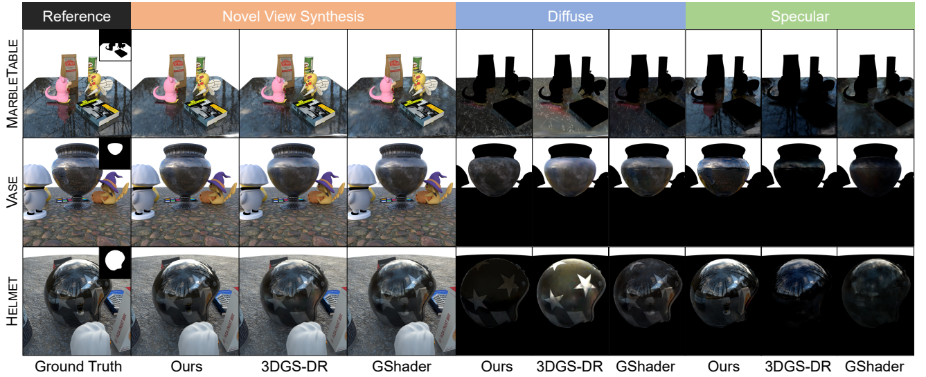
Figure 4. Novel view synthesis and image decomposition results on synthetic scenes, comparing our SpecTRE-GS with 3DGS-DR [39] and GShader [13]. SpecTRE-GS better distinguishes diffuse and specular components in reflective regions, with the least baked-in view-dependent appearance in diffuse components. The masks of reflective regions are shown as insets in the reference image.
