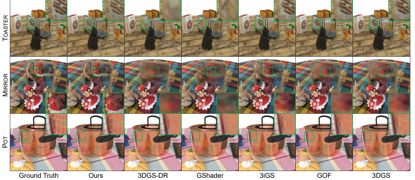
Figure 3. Novel view synthesis comparison on synthetic scenes. We evaluate SpecTRE-GS against relevant 3DGS-based methods modeling view-dependent appearances: 3DGS-DR [39], GShader [13], 3iGS [30], GOF [42], and 3DGS [15]. The insets highlight the improvement of SpecTRE-GS in rendering high-frequency specular reflections, showcasing the precise positioning of reflected content and sharp details.
