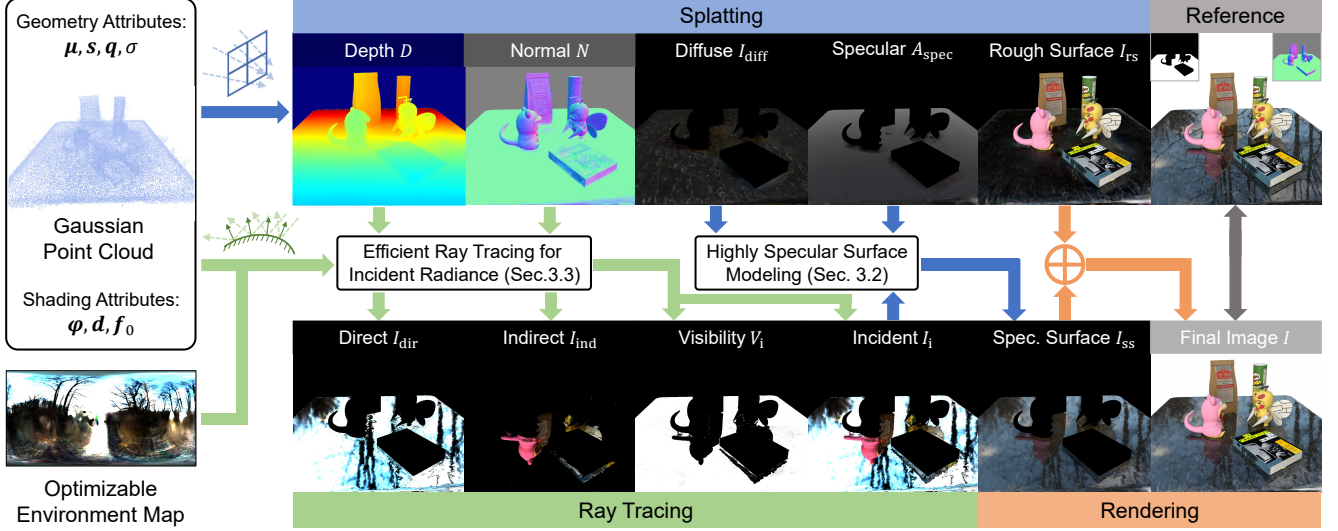
Figure 2. Overview of the SpecTRE-GS pipeline. The scene is represented as a Gaussian point cloud, where each Gaussian is associated with geometry and shading attributes used to render the depth map D , normal map N , diffuse reflection I_{\text{diff}} , specular reflectance A_{\text{spec}} , and rough surface reflection I_{\text{rs}} through splatting (Sec. 3.1). Highly specular surface reflection I_{\text{ss}} is formulated as the sum of the diffuse reflection I_{\text{diff}} and the specular reflection computed from the incident radiance I_i and specular reflectance A_{\text{spec}} (Sec. 3.2). The incident radiance I_i is determined along reflected secondary rays given by the scene geometry D and N , with the indirect component I_{\text{ind}} and visibility V_i evaluated via efficient ray tracing within the Gaussian point cloud, and the direct component I_{\text{dir}} modeled by an optimizable environment map (Sec. 3.3). The scene geometry is enhanced using normal prior guidance, numerical gradients from ray-traced incident radiance, and other training signals to achieve undistorted reflections (Sec. 3.4).
