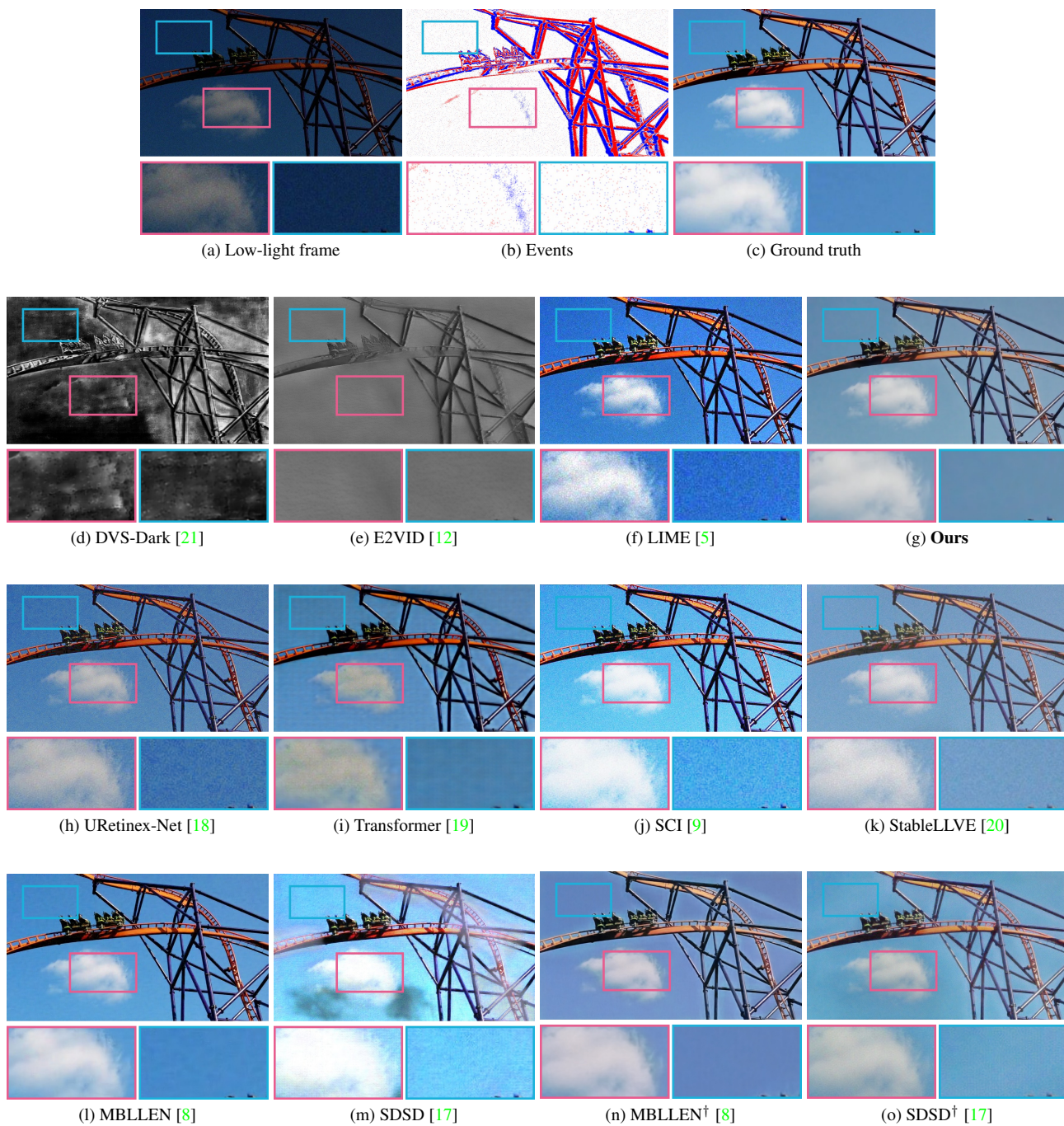
Figure 11. Visual comparison results with state-of-the-art methods on synthetic data.
