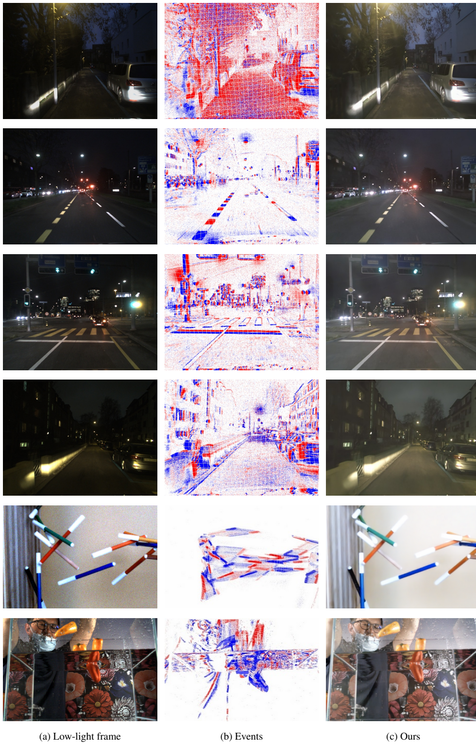
Figure 14. Visual results on real data captured in DSEC [3] (the first four rows) and Time Lens [16] (the last two rows).
